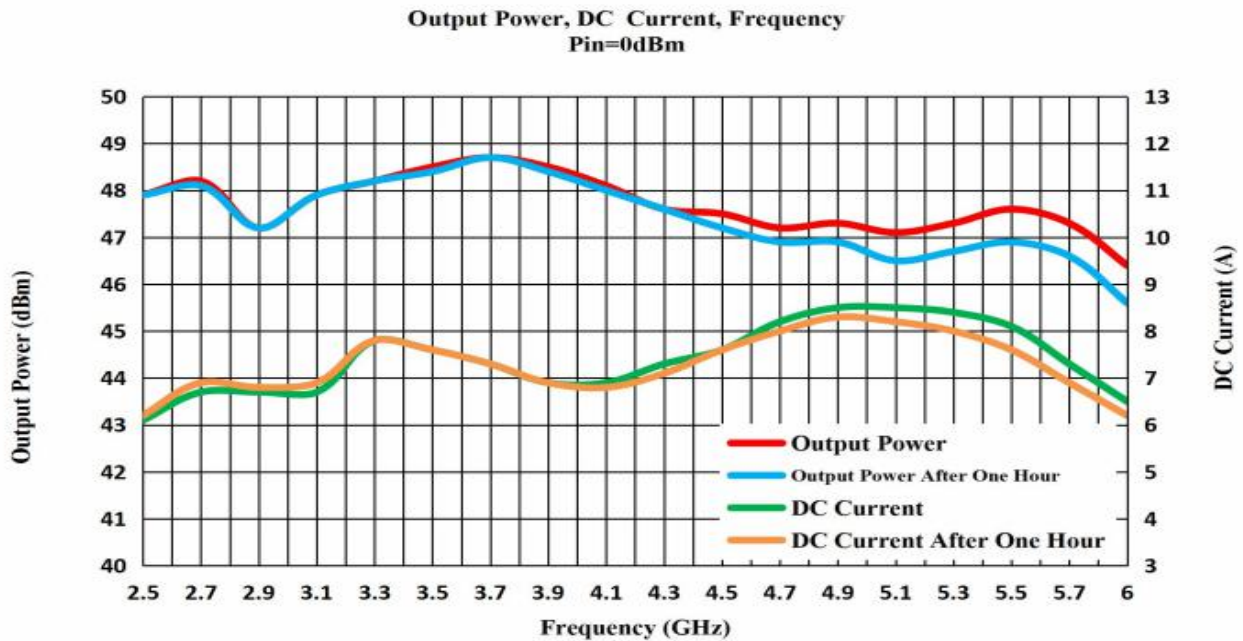
Graph 2: Output Power (High temp. +60±3°C)
