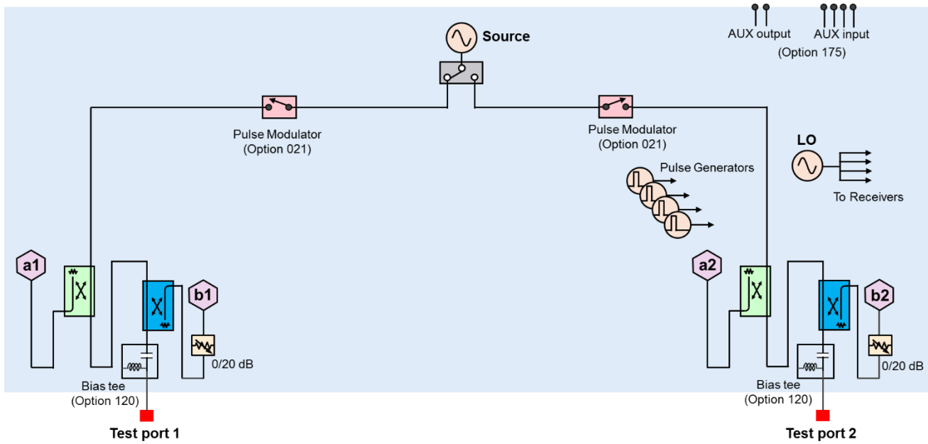
E5080B Option 240/260/290/2D0/2K0 (2-port base options)
