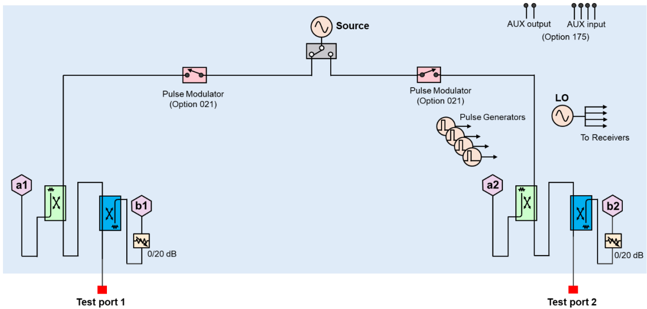
E5080B Option 2L0/2M0/2N0/2P0 (2-port base options)
