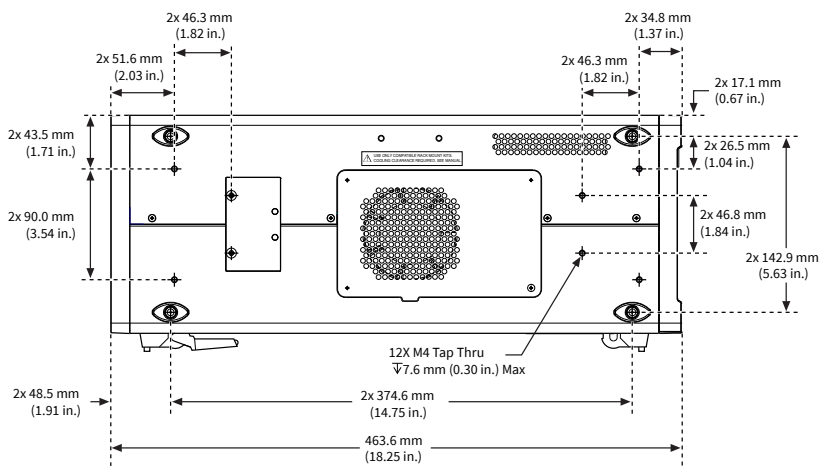
Figure 1. PXIe-1092 Chassis Dimensions (Side)
