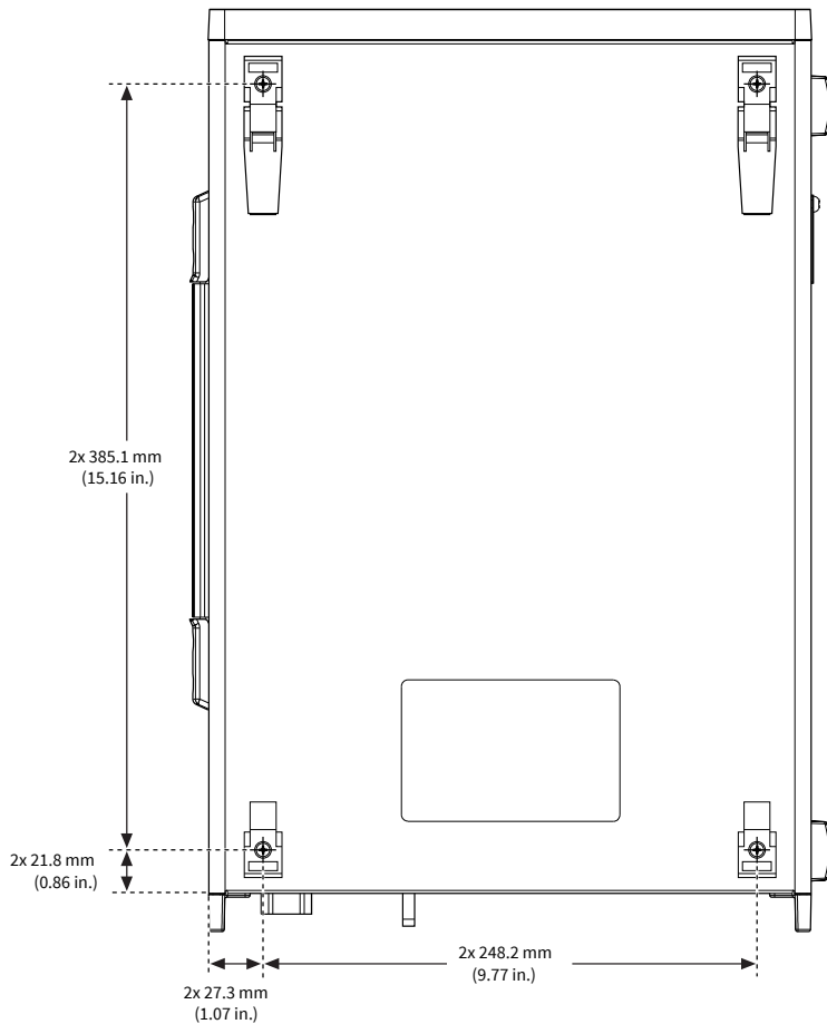
Figure 1. PXIe-1092 Chassis Dimensions (Bottom)
