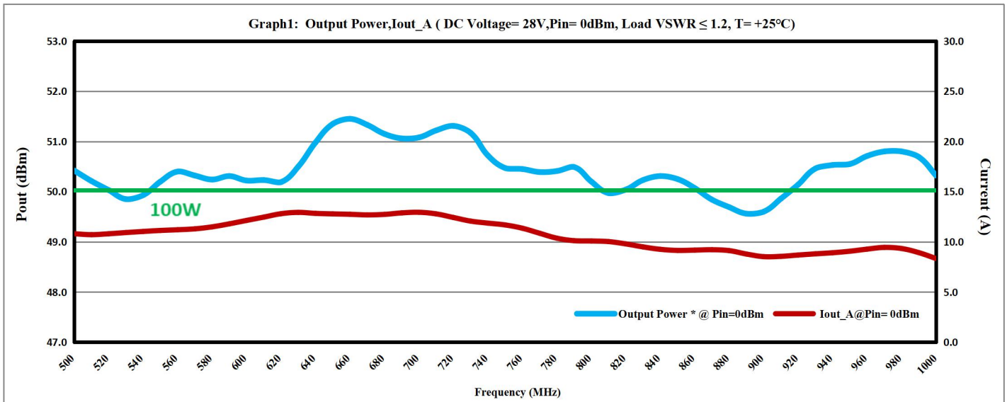
Pout and Iout Curve with Pin=0dBm(CW)
