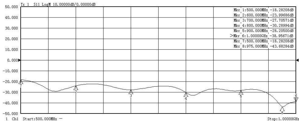
S21 Curve, Pin=0dBm (Up) & S11 Curve, Pin=-30dBm(Down) [Load VSWR ≤ 1.2]
