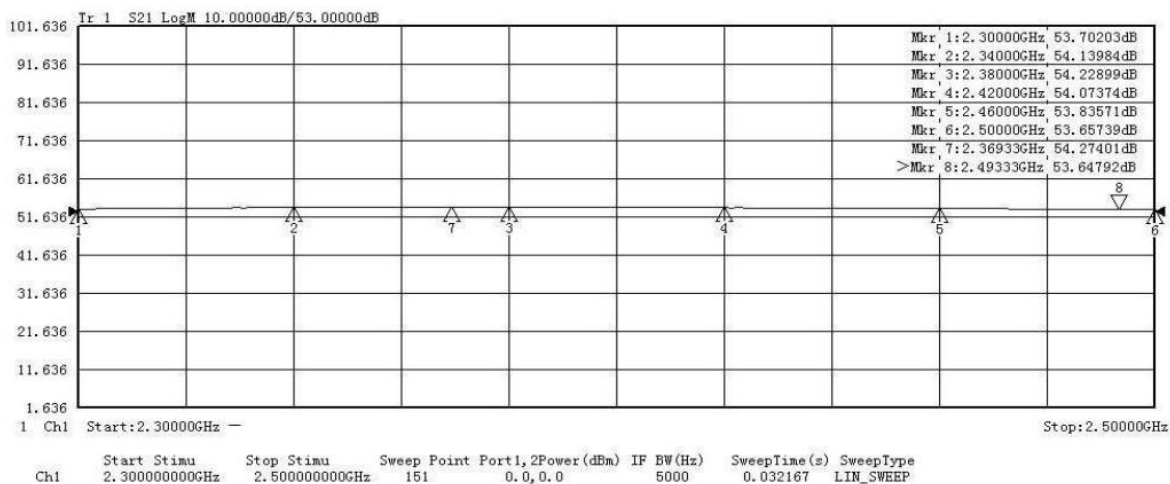
Graph 2: Power Gain (Voltage=28V, Load VSWR≤1.2, 25°C)
