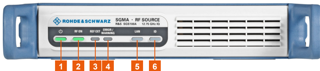
Figure 5-1: R&S SGS front panel controls
