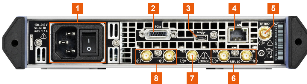
Figure 5-2: R&S SGS rear panel controls and connectors
