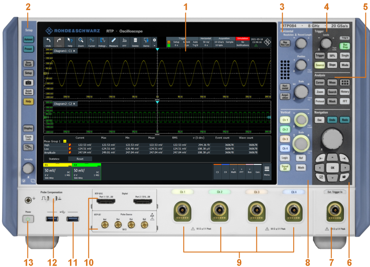
Figure 5-1: Front panel of R&S RTP
