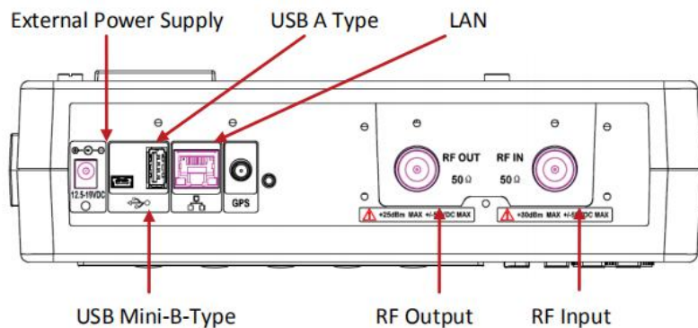
Fig.2.2 S5800E test panel connector overview
