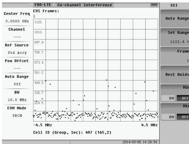
Fig.5.70 One frame
