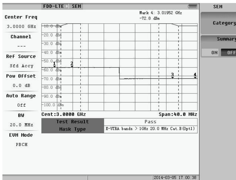
Fig.5.68 Summary closed
