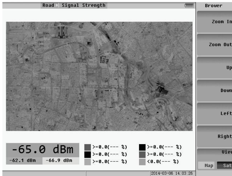
Fig.6.20 Satellite map
