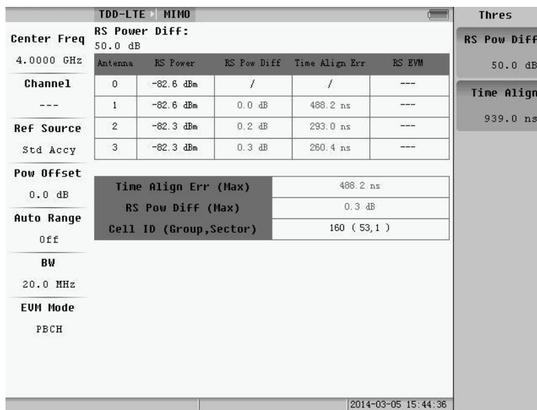
Fig.5.38 Thres submenu
