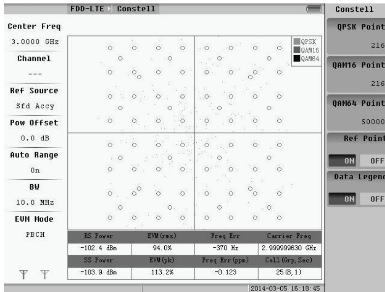
Fig.5.49 Constellation menu
