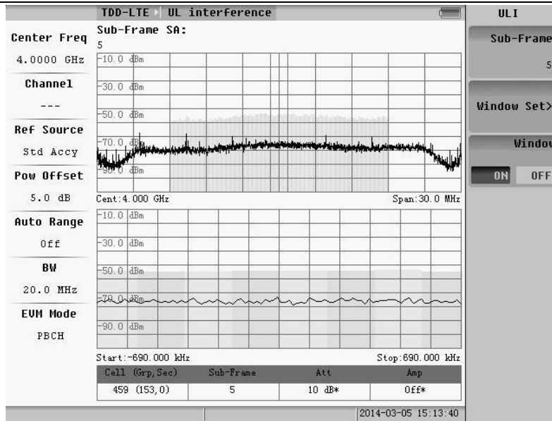
Fig.5.34 ULI menu
