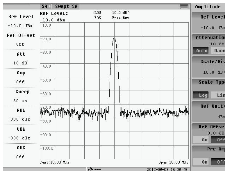
Fig.3.16 Scale is 10 dB/ in logarithmic state (default value)
