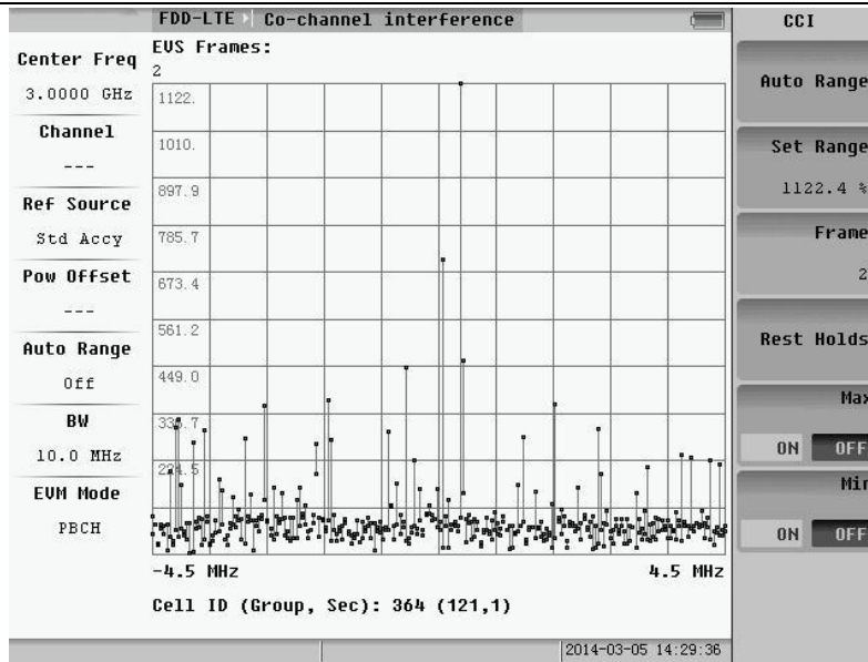
Fig.5.69 CCI menu
