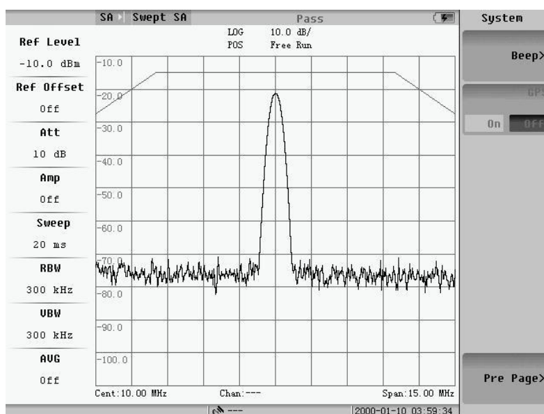
Fig.9.17 GPS setting
