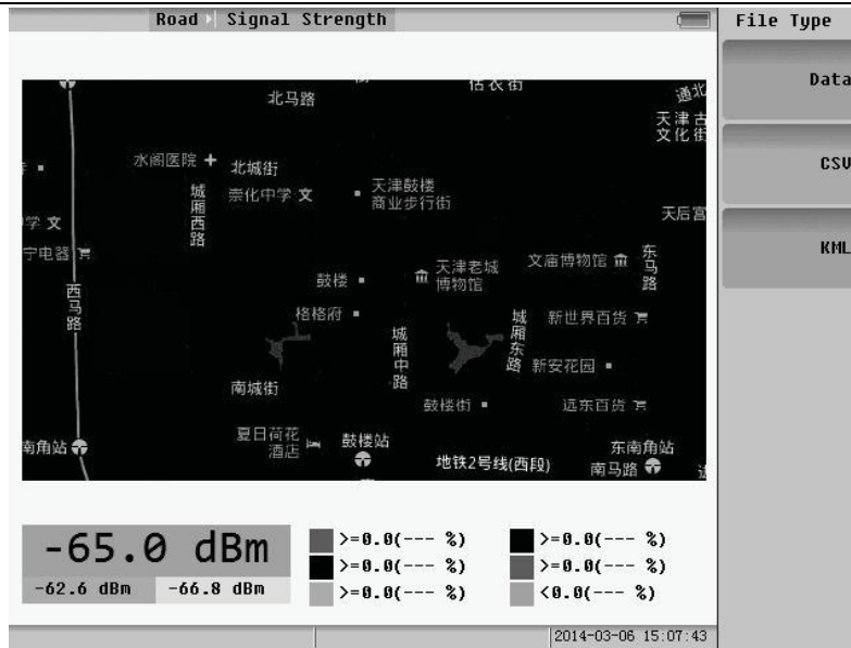
Fig.6.23 File type
