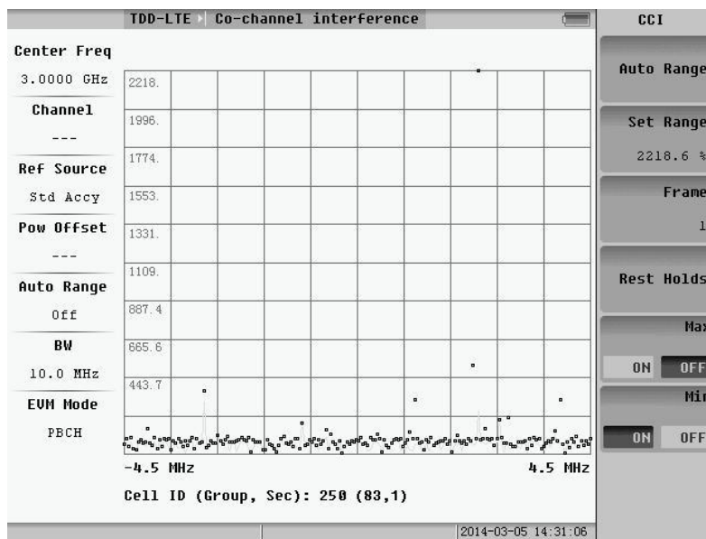
Fig.5.33 Min. holds
