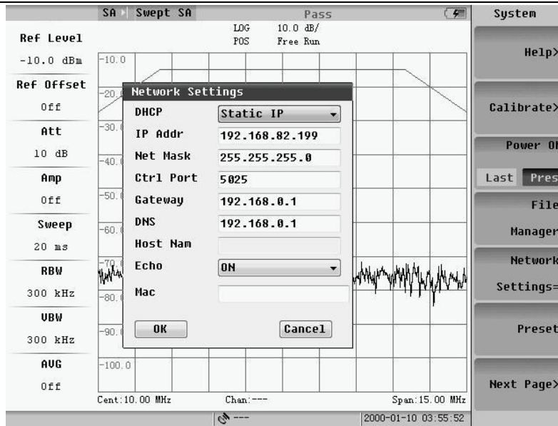
Fig.9.12 Network setting
