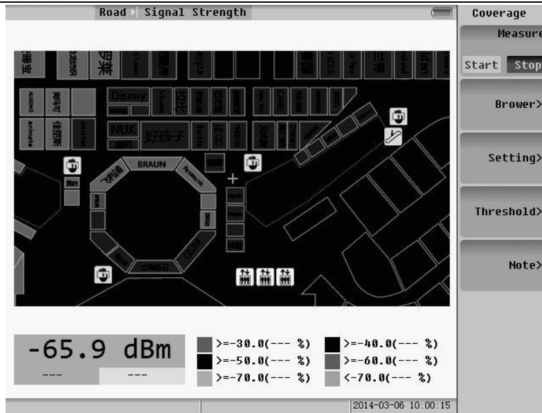
Fig.6.3 Measure stop
