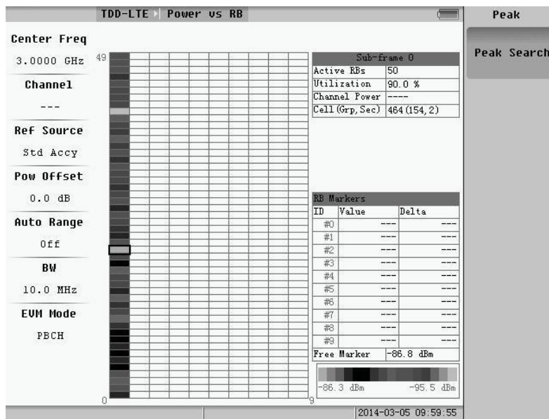
Fig.5.11 Peak search
