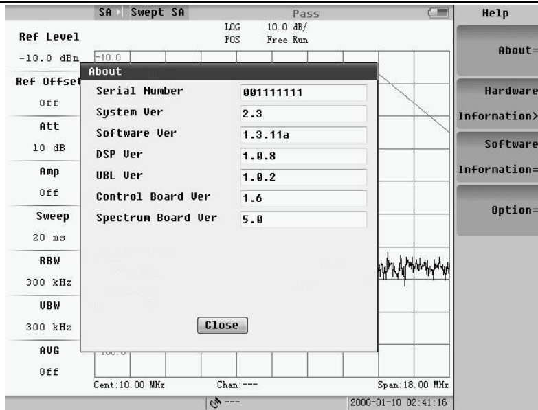
Fig.9.7 Instrument information
