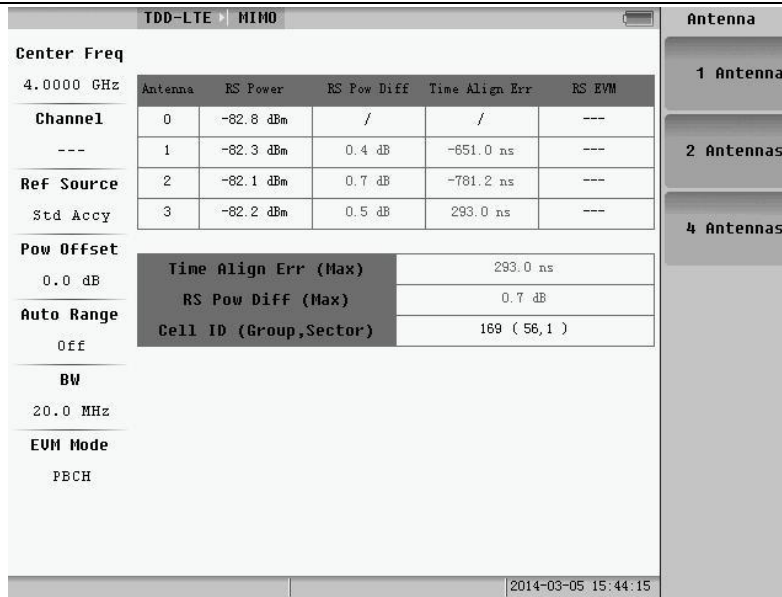
Fig.5.38 Antenna submenu
