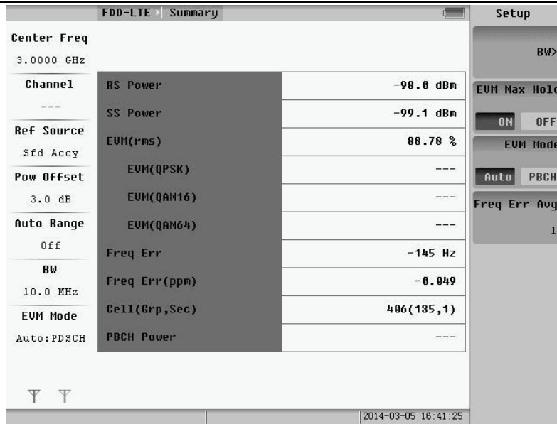
Fig.5.55 Summary measure
