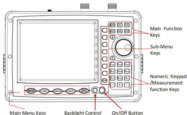
Fig.2.1 S5800E overview
