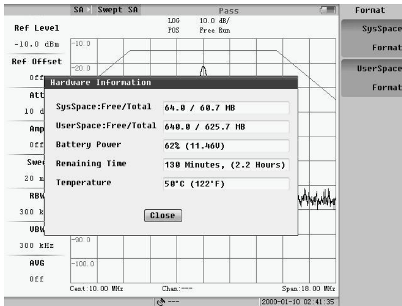
Fig.9.8 Hardware information
