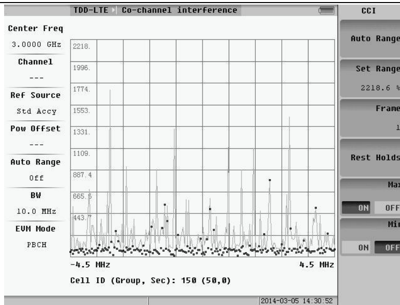
Fig.5.32 Max. holds
