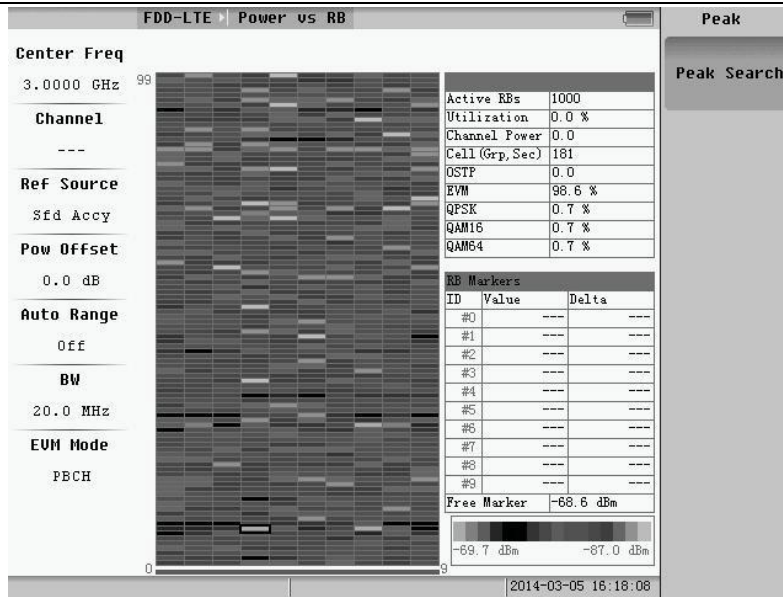
Fig.5.48 Peak search
