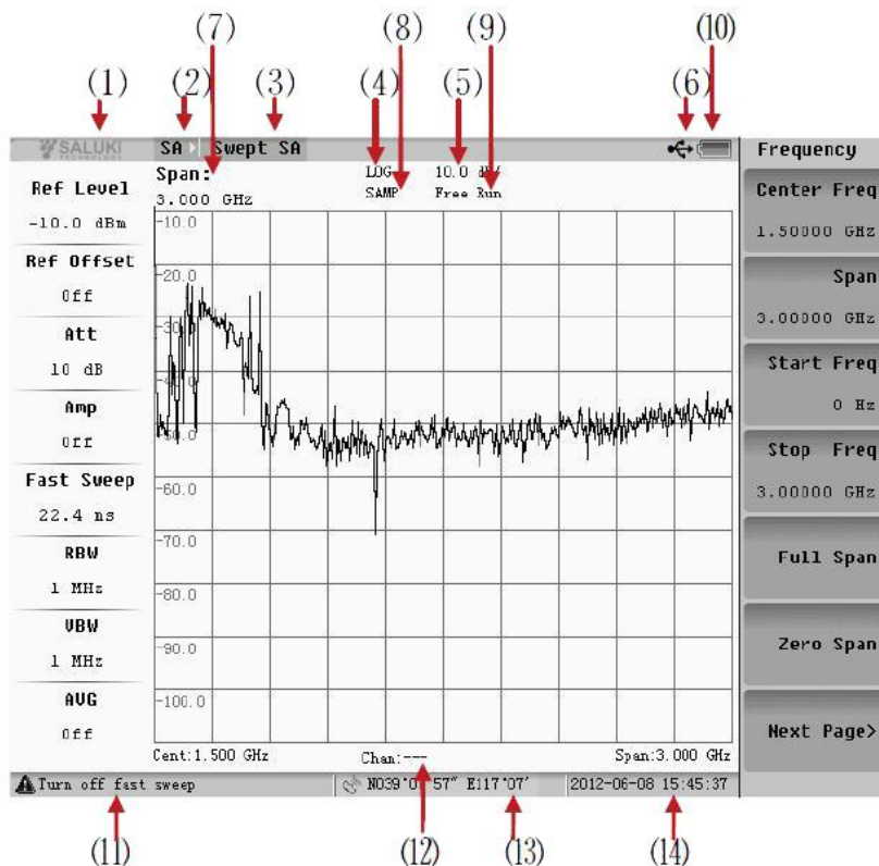
Fig.2.3 Screen information
