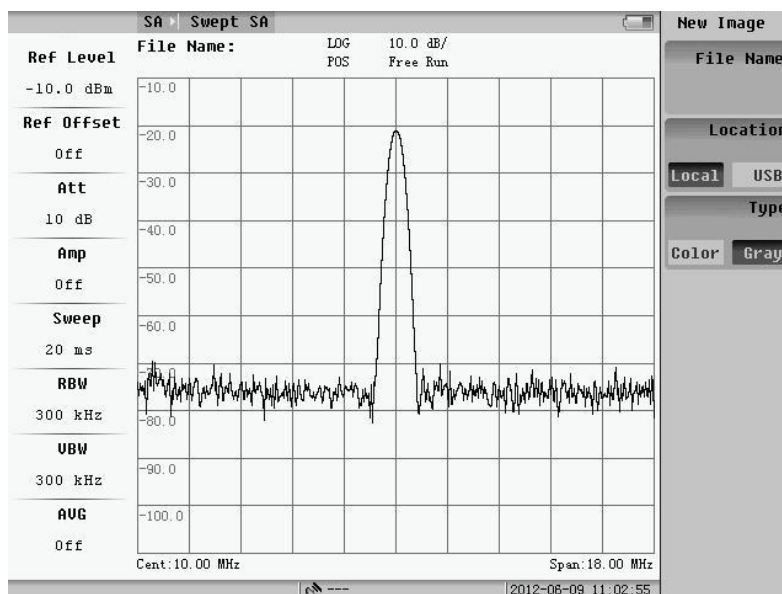
Fig.8.2 Image saving
