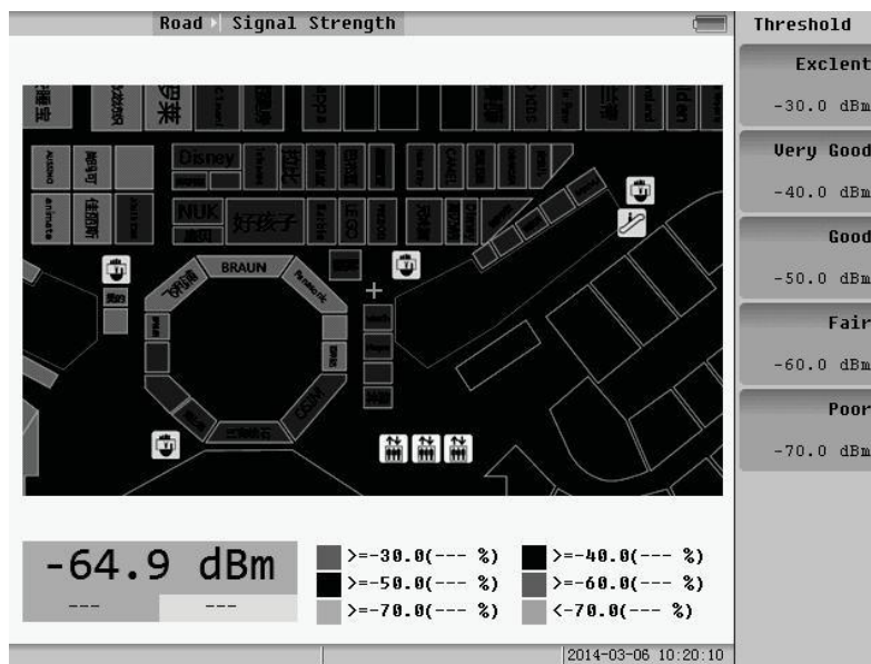
Fig.6.6 Threshold menu
