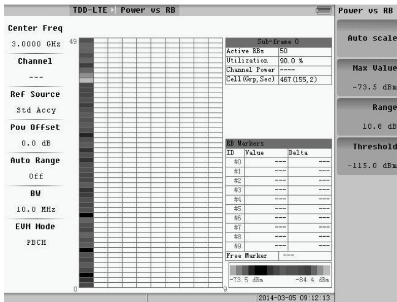
Fig.5.6 Auto scale
