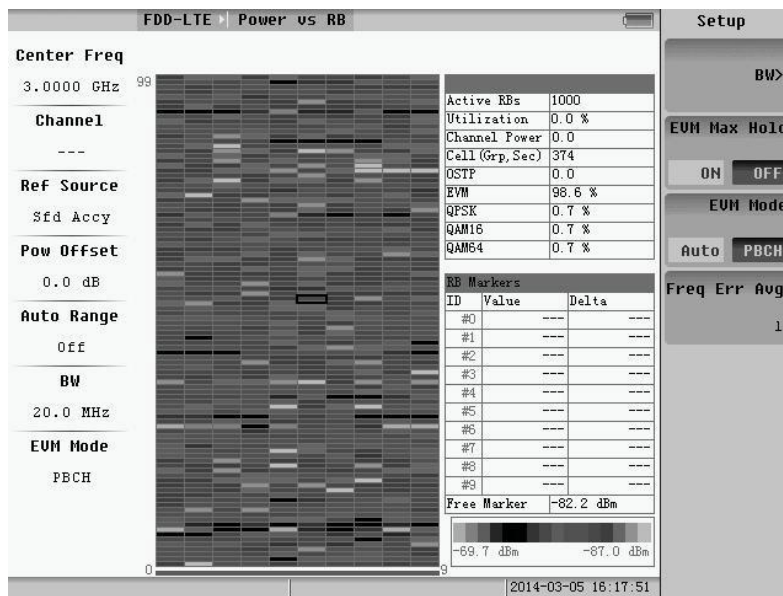
Fig.5.47 Setup
