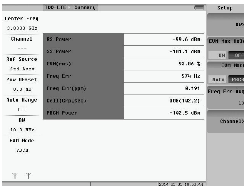
Fig.5.17 Summary measure
