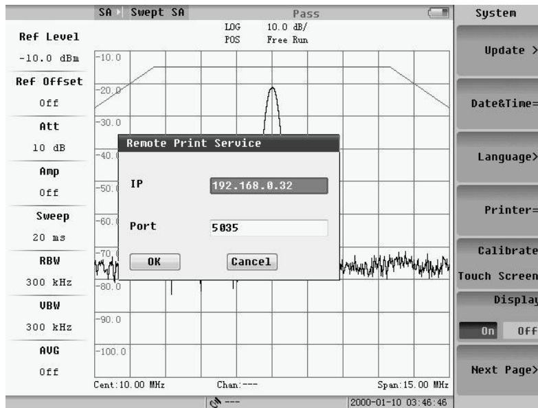
Fig.9.14 Printer setting
