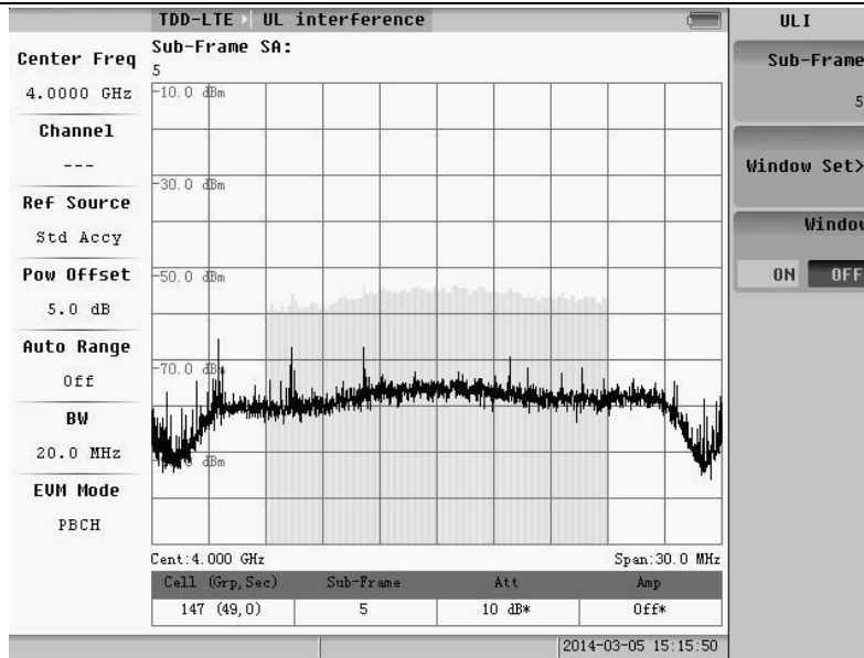
Fig.5.36 Window closed
