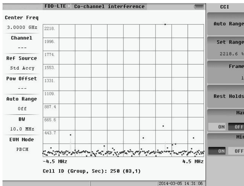
Fig.5.72 Min holds
