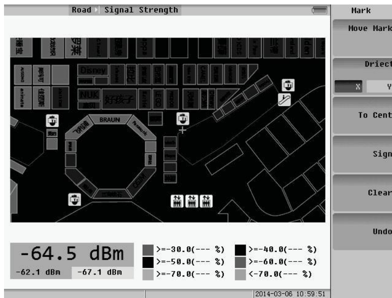
Fig.6.8 MARK menu
