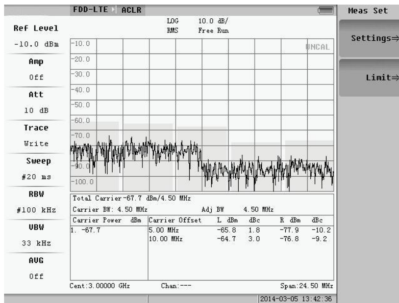
Fig.5.64 ACLR menu
