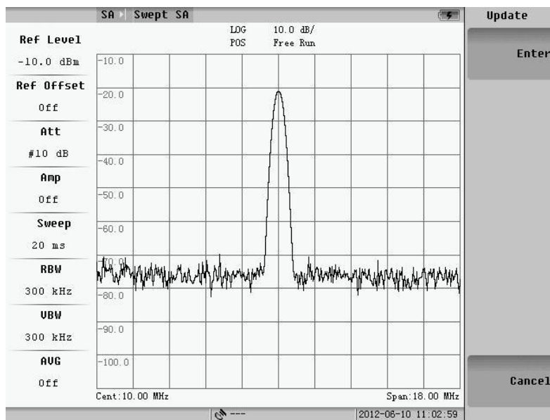
Fig.9.18 Upgrade
