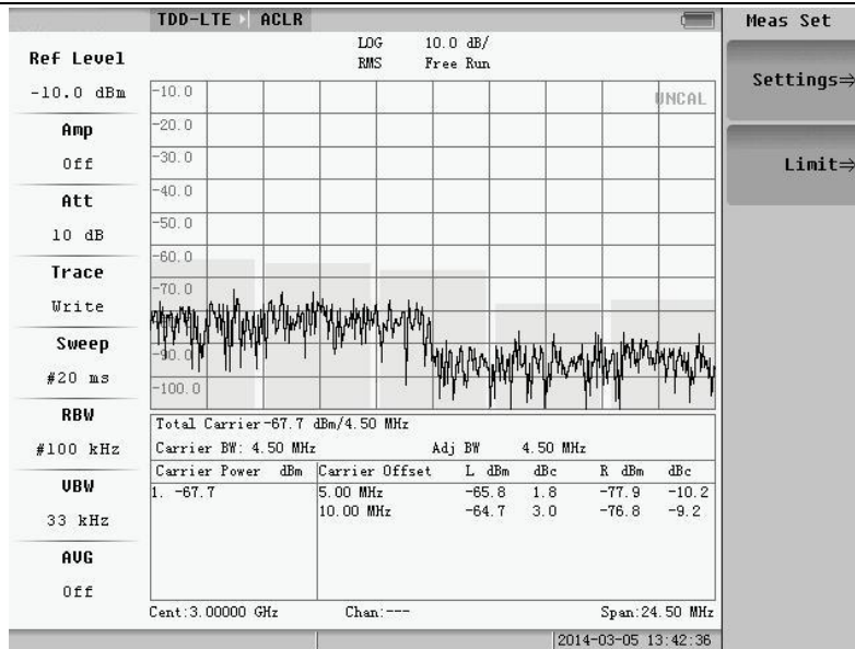
Fig.5.26 ACLR menu
