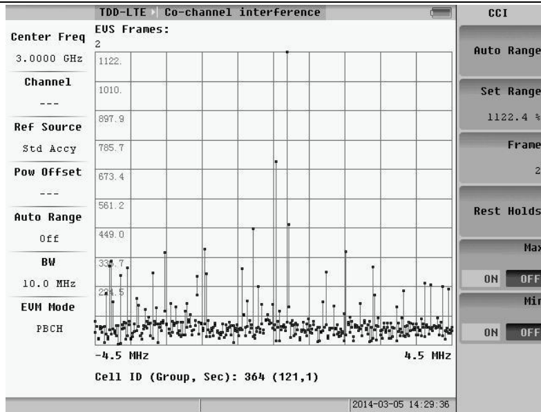
Fig.5.30 CCI menu
