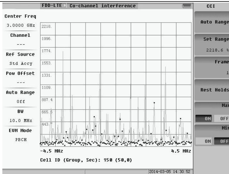
Fig.5.71 Max holds
