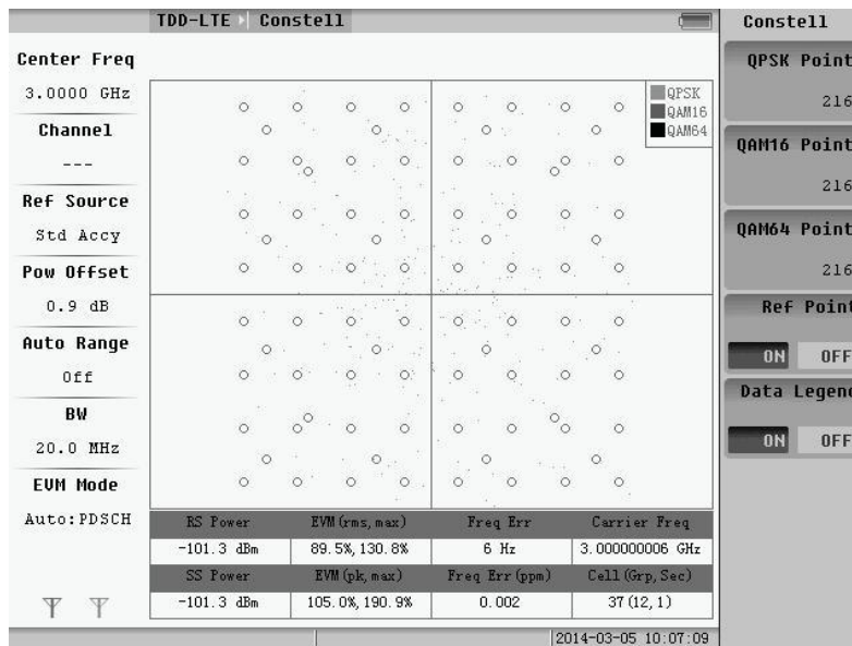
Fig.5.12 Constellation menu
