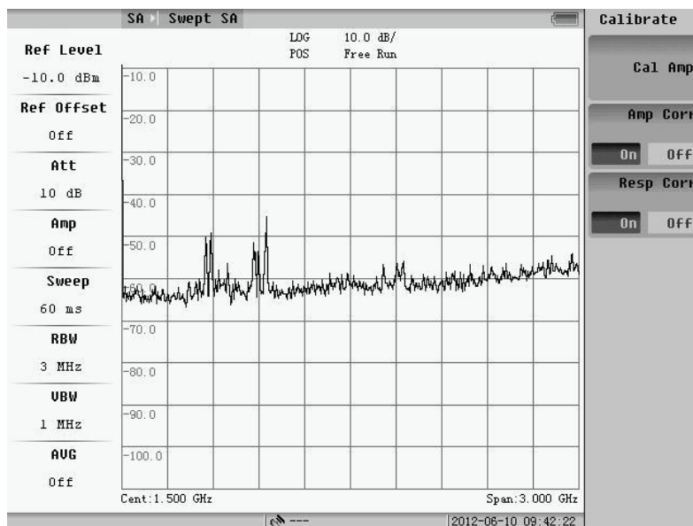
Fig.9.4 Calibration menu
