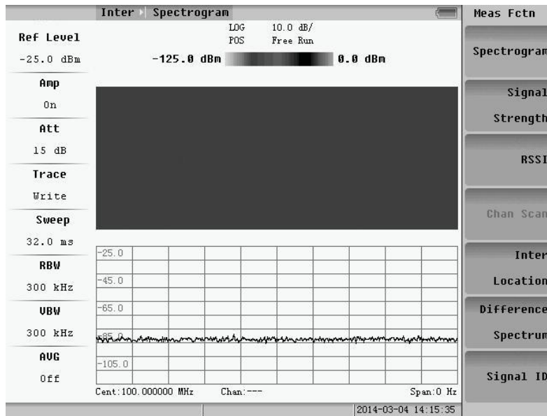
Fig.4.1 Interference analysis
